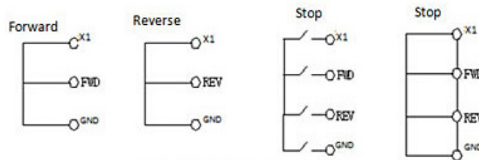
3 lines control mode description
