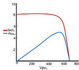
■ I-V characteristics
