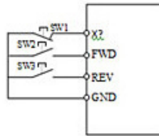
a) 3 lines control mode 1
