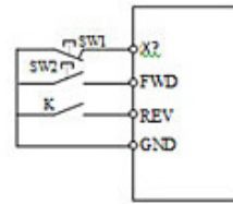
b) 3 lines control mode 2
